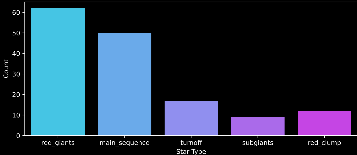
APOGEE DR17 Field: [040+60] Count plot of Star Type
