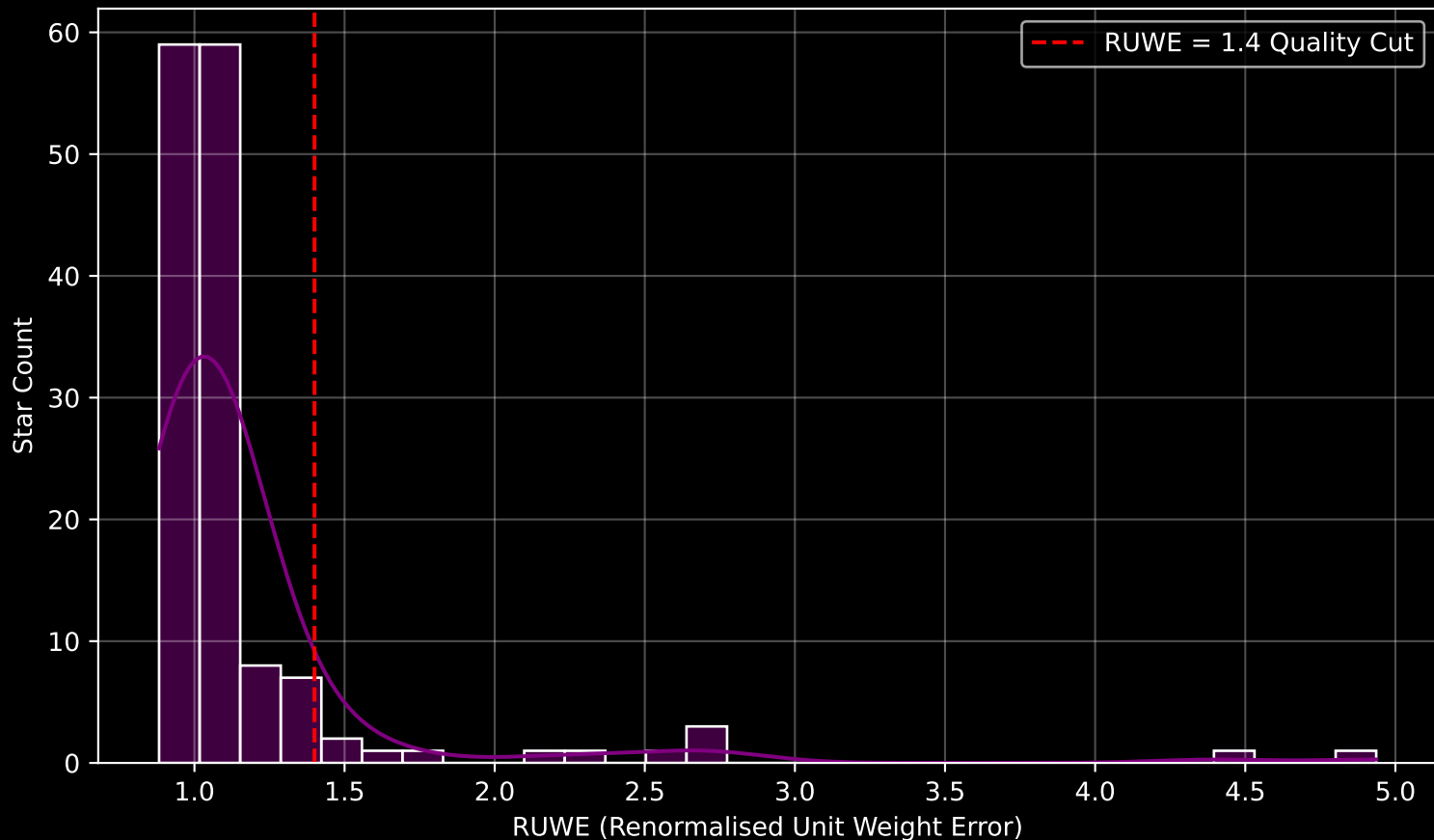
GAPOGEE DR17 Field [040+60] RUWE Distribution (n= 145)
