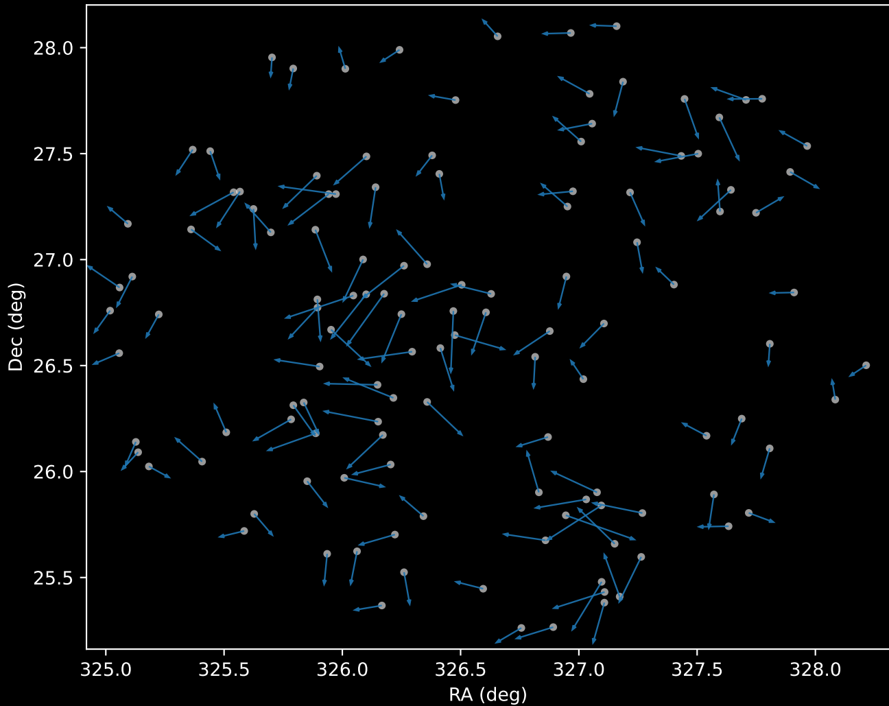
APOGEE DR17 Cluster 0 Proper Motion Vectors (n=124)
