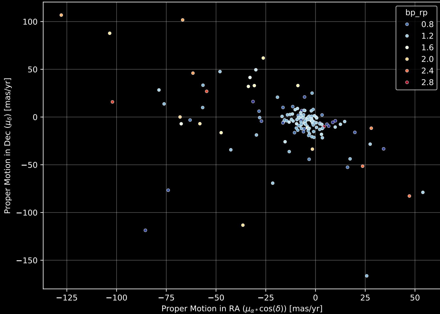
APOGEE DR17 Field: [040+60] Proper Motion Diagram (n= 150)
