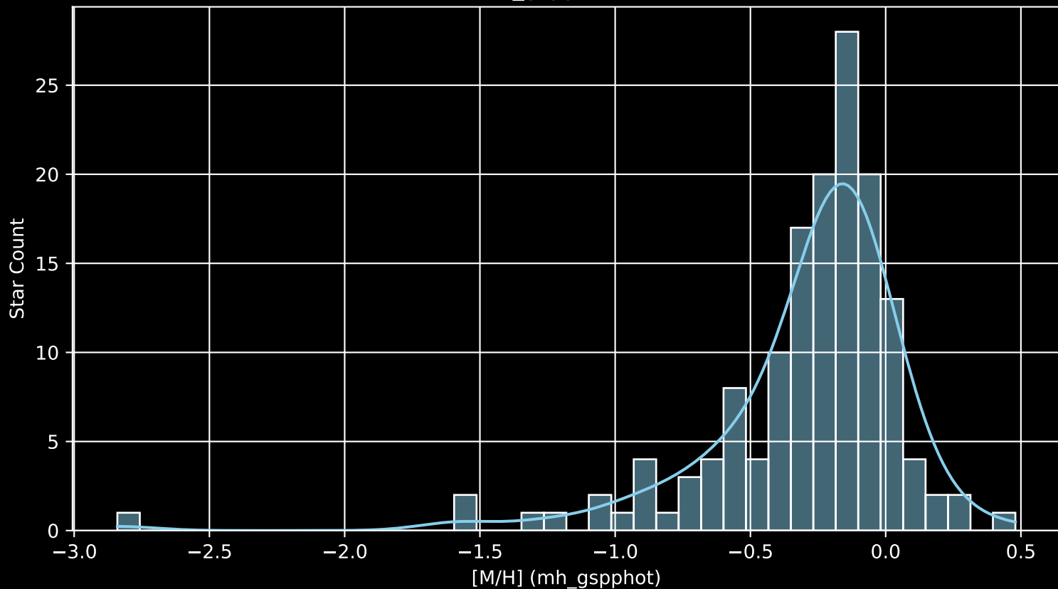
APOGEE DR17 Field: [040+60 [M/H] (mh_gspphot) (n= 149)
