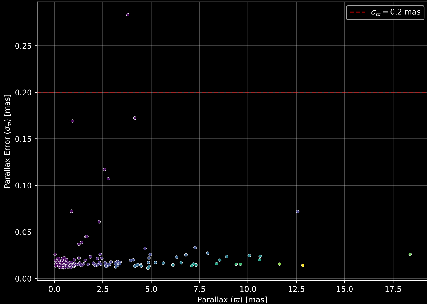
APOGEE DR17 Field: [040+60] Parallax Quality (n= 150)
